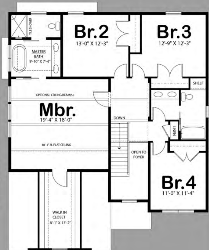
Second Level
